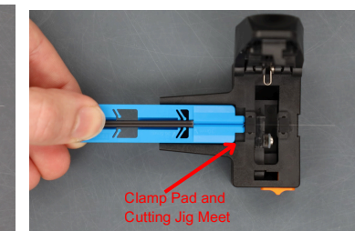
Step 8: Slide the cutting jig in the holder slot of the cleaver until it meets the clamp pad. Cleave fiber.
